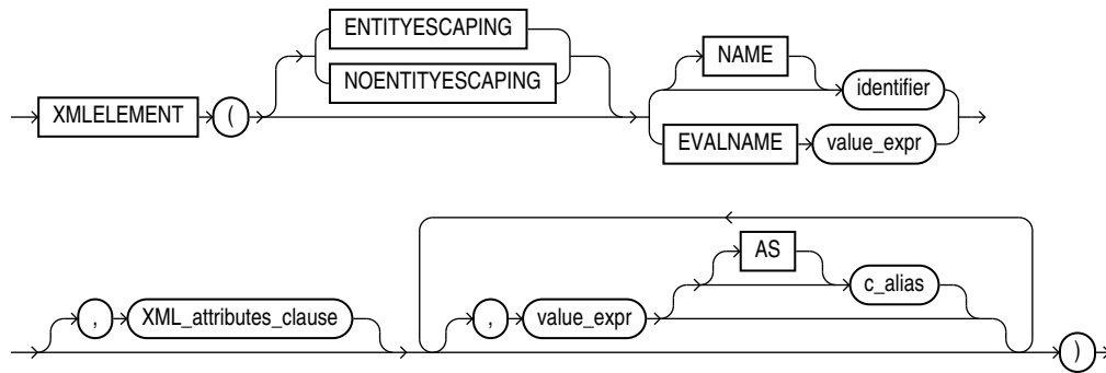
Figure 8-1 XMLLEMENT Syntax
