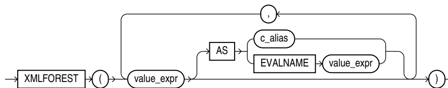
Figure 8-3 XMLFOREST Syntax
