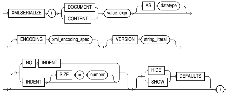
Figure 8-8 XMLSerialize Syntax
