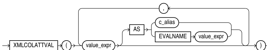
Figure 8-10 XMLCOLATTVAL Syntax
