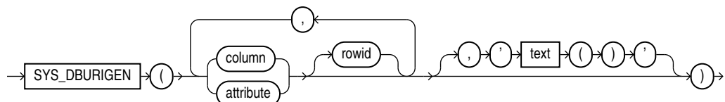
Figure 32-2 SYS_DBURIGEN Syntax
